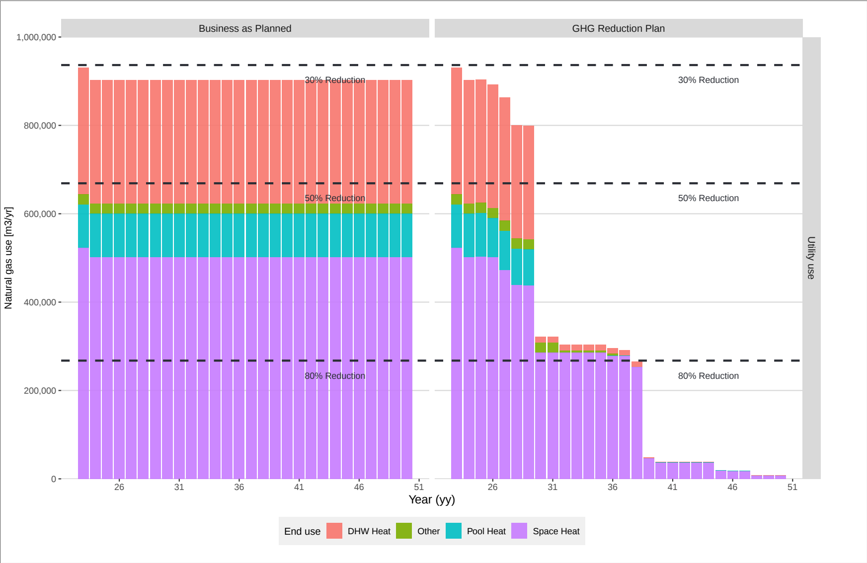
Figure 4: Natural Gas Utility Use Projection for Each Scenario
