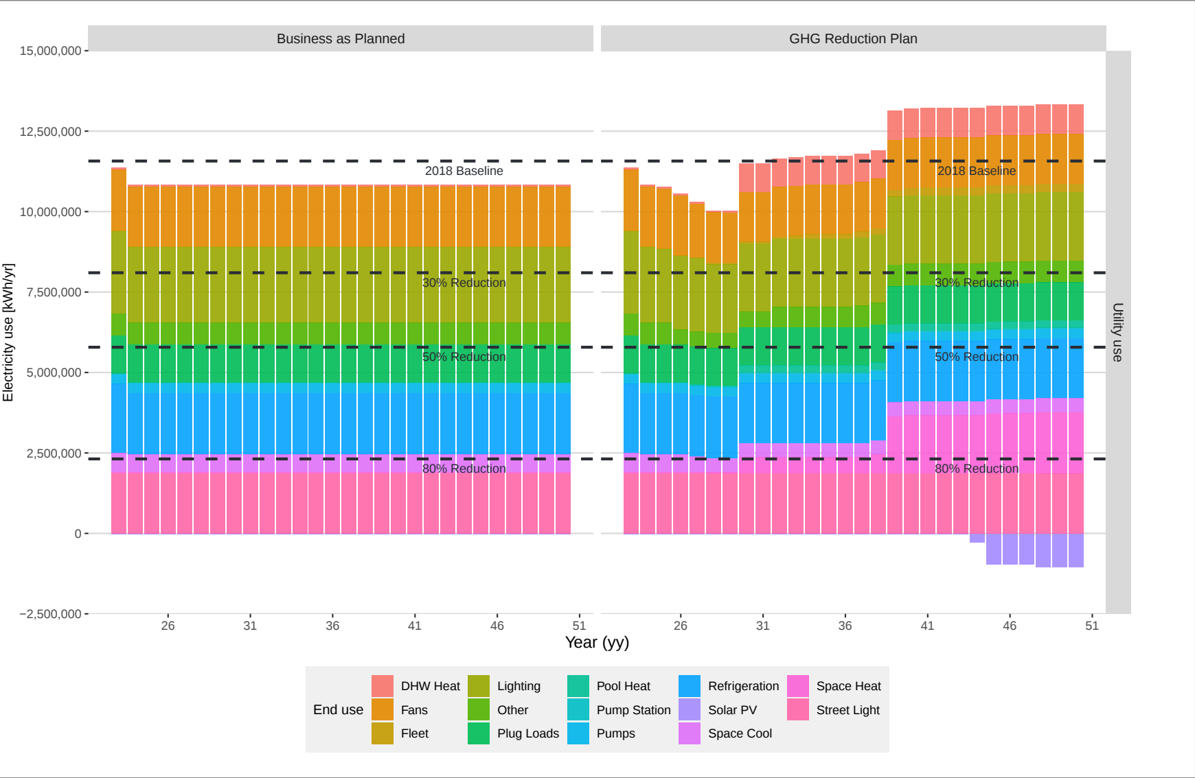
Figure 3: Electricity Utility Use Projection for Each Scenario
