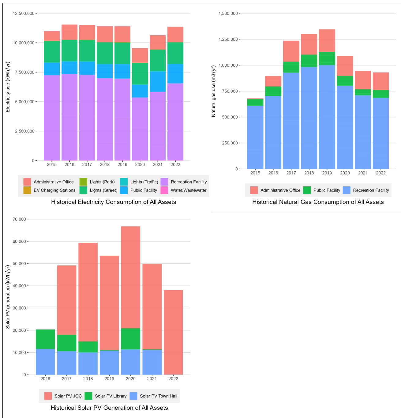
Figure 3: Buildings Historical Energy Use.
