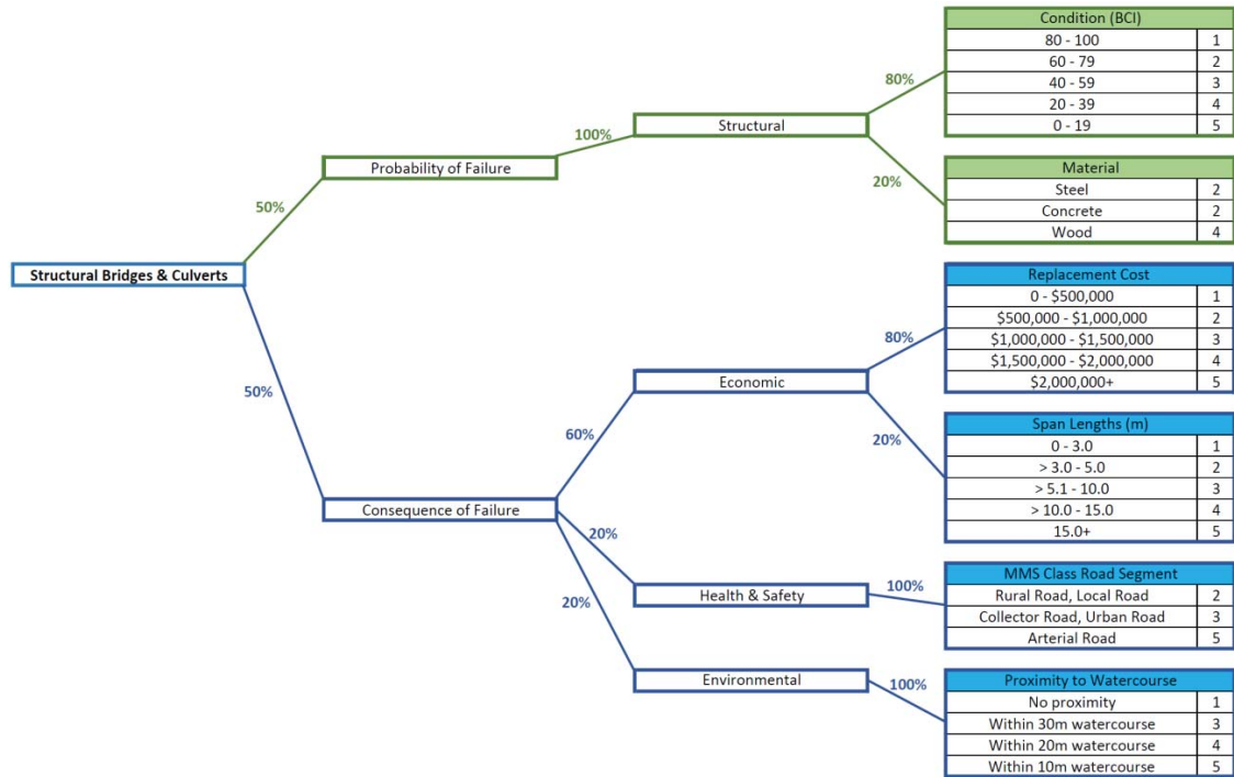
Figure 97 Bridges and Culverts Risk Rating Criteria
