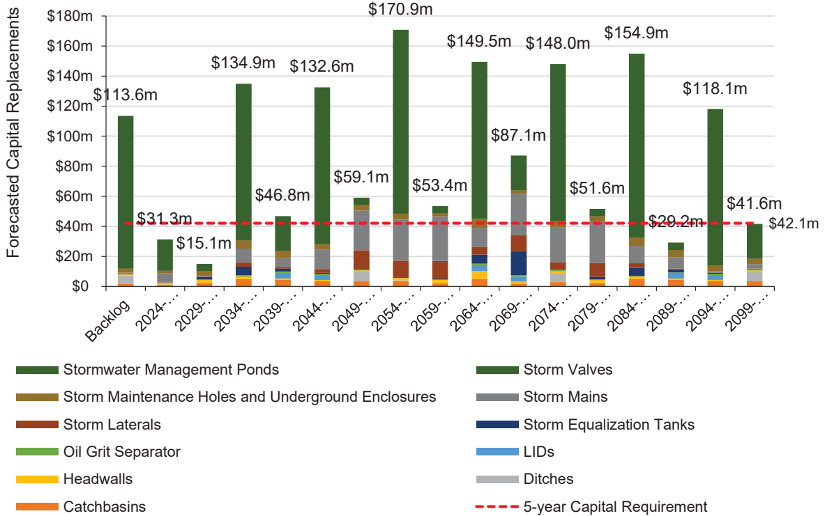
Figure 58 Storm Network Forecasted Replacement Needs 2024-2103
