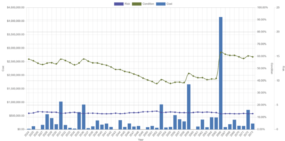
Figure 68 Storm Network (Headwalls) Proposed LOS Impacts
