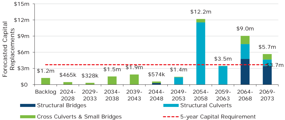
Figure 23 Bridges and Culverts Forecasted Replacement Needs 2024-2073
