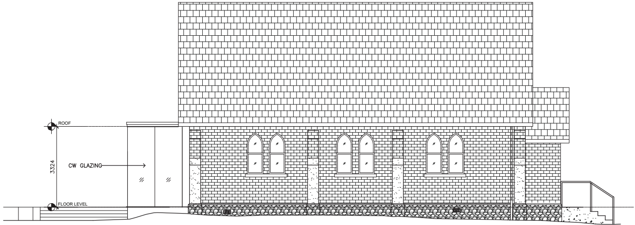
EAST elevation 2
