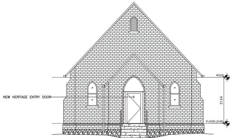
NORTH elevation 1
